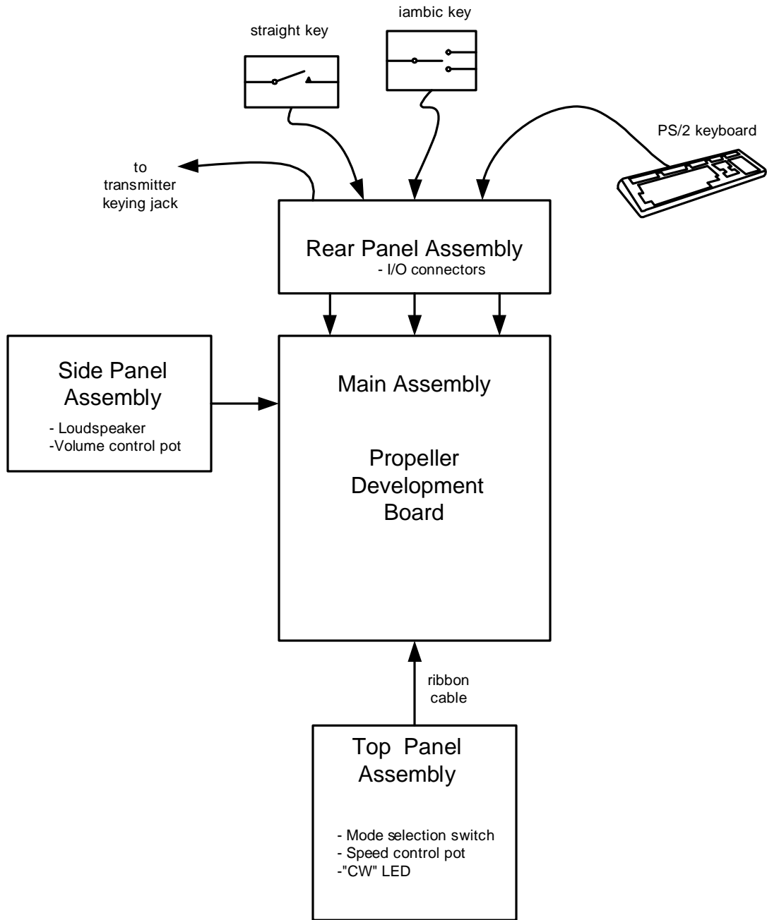
PropKeyer Hardware Block Diagram
